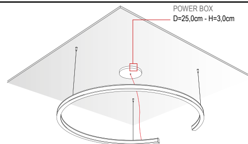
KRONOS CON BOX KRONOS WITH POWER SUPPLY BOX
