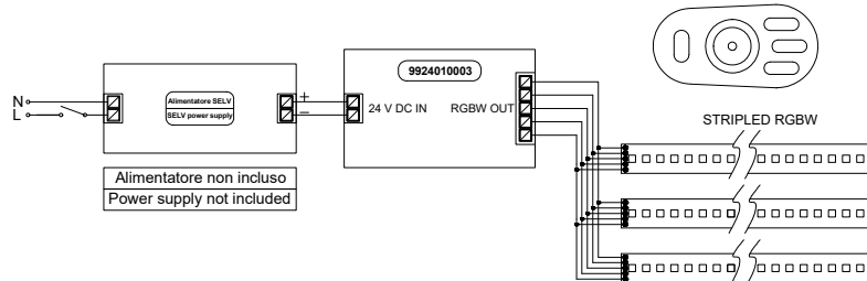
Schema collegamento CONTROLLER RGBW + RADIOCOMANDO art.: Wiring diagram RGBW CONTROLLER + REMOTE TOUCH CONTROL ref.:
